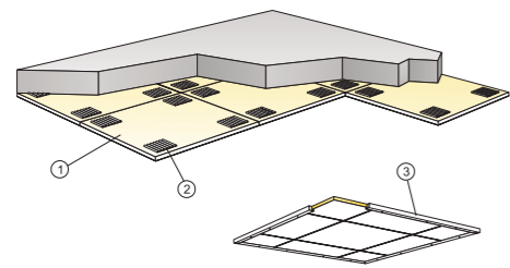
M03 Installation diagram (M03) for Ecophon Focus B, using Connect Absorber glue
