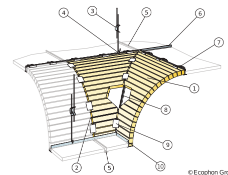
Installation diagram (M31EC) for Ecophon Focus Flexiform A external corner
