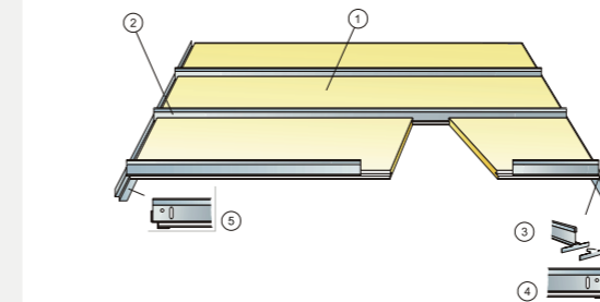
Installation diagram (M17) for Focus D/A in corridor
