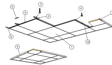
Installation diagram (M15) for Ecophon Focus F
