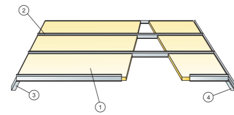
M16 Installation diagram (M16) for Ecophon Focus A XL in corridors
