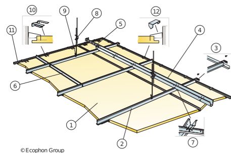
M207 Installation diagram (M207) for Ecophon Focus Ds 1200x1200 mm
