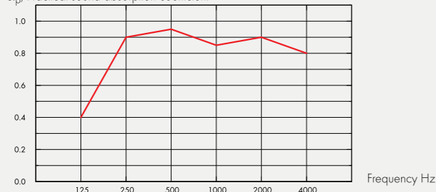
\alpha_p , Practical sound absorption coefficient
