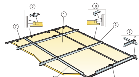
M208 Installation diagram (M208) for Ecophon Focus Ds, direct installation
