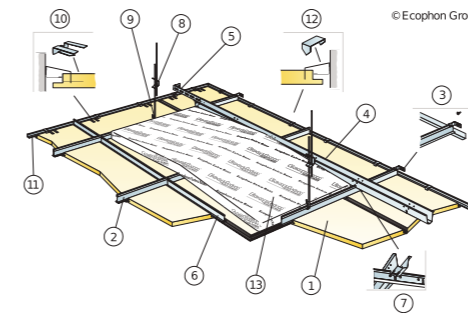
M400 Installation diagram (M400) for Ecophon Focus Ds
