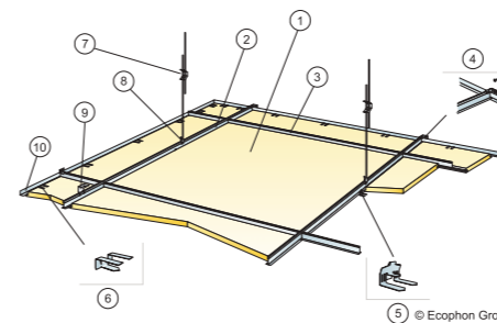
M203 Installation diagram (M203) for Ecophon Focus Dg 1200x1200 mm
