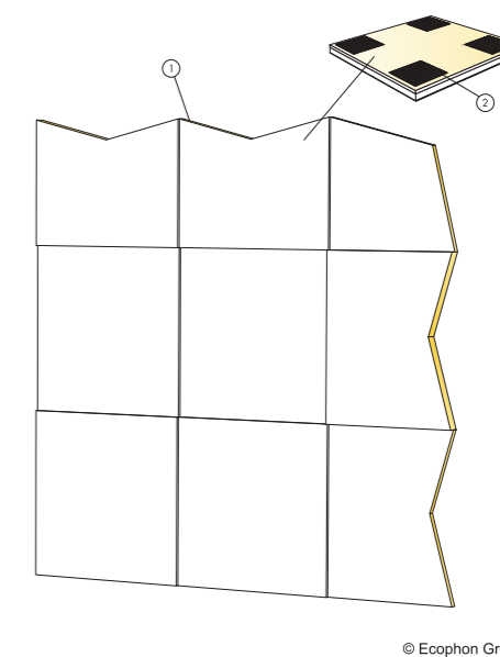
M489 Installation diagram (M489) for Ecophon Focus Levels, using Connect Absorber glue
