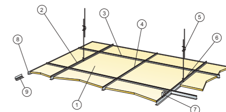
M01 DIN Installation diagram (M01) for Ecophon Focus A
