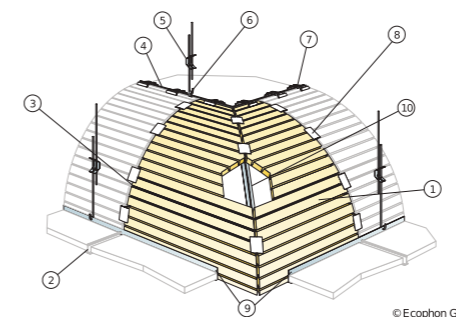
Installation diagram (M31IC) for Ecophon Focus Flexiform A internal corner
