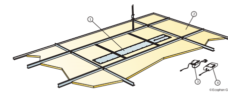
M519 Installation diagram (M519) for Ecophon Line LED Dg and E
