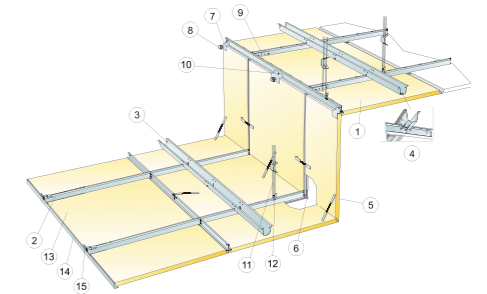
M394 Installation diagram (M394) for Ecophon Focus Ds Level change
